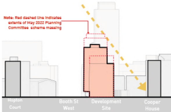
Current August 2022 Scheme - North-South Site Section Diagram
